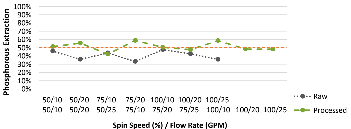
Graph 3: P Extraction from Raw & Processed Manure (flush barn)
