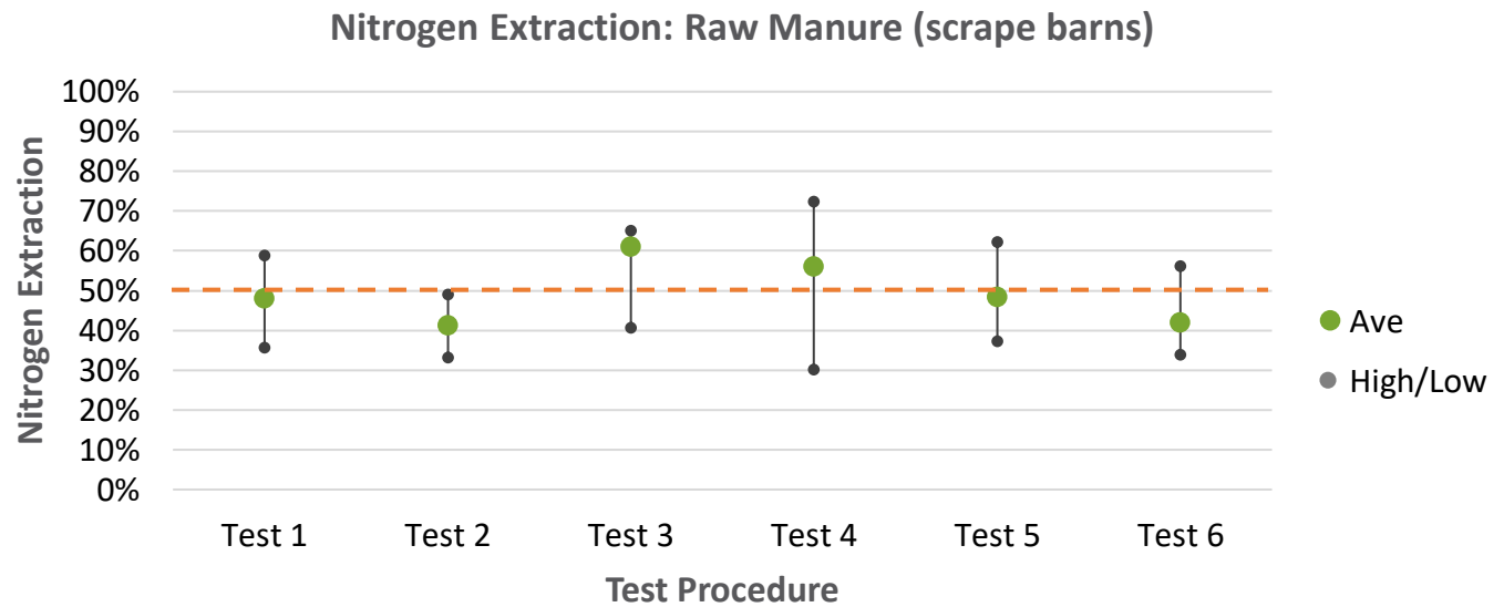
Graph 4: Nitrogen Extraction from Raw Manure (scrape barns)
