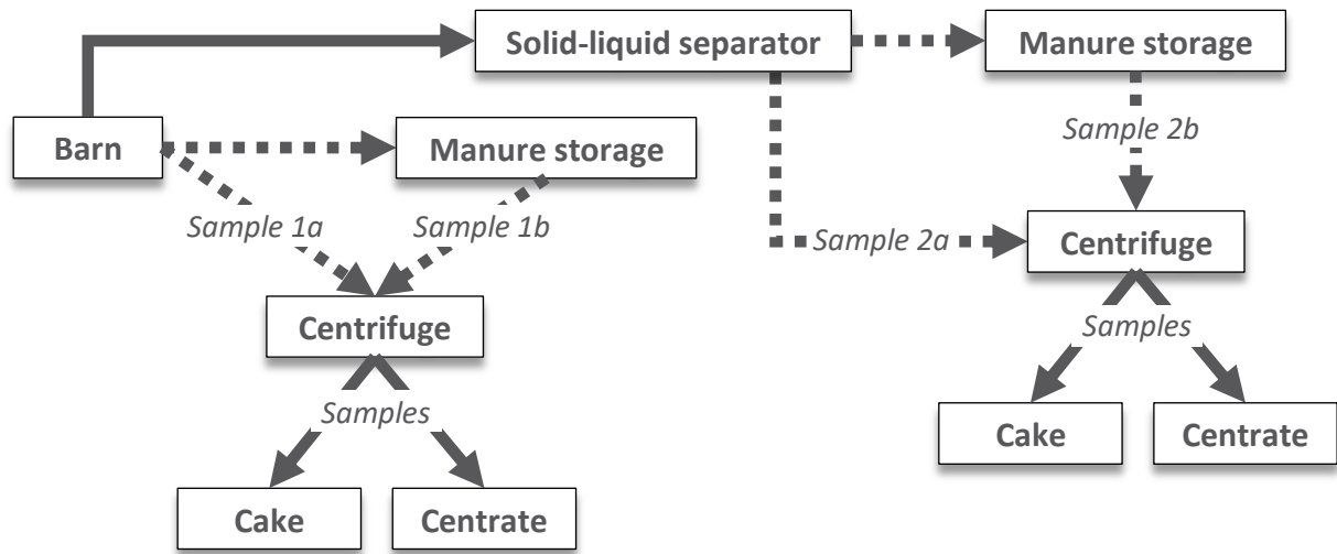
Figure 4: Test Set-Up
