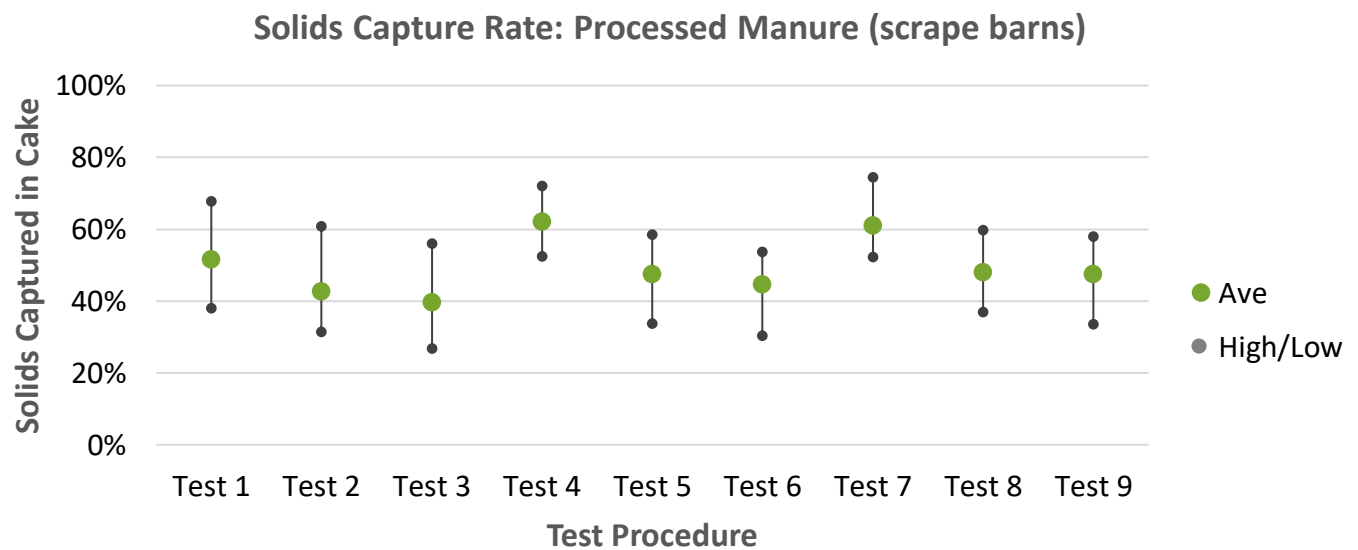
Graph 11: Solids Capture from Processed Manure (scrape barn)
