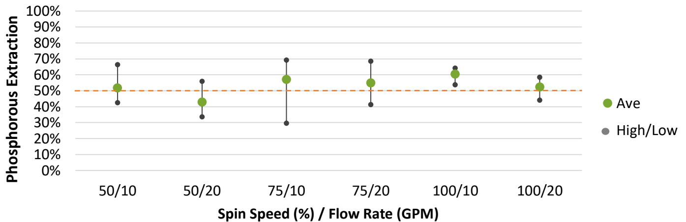
Graph 1: P Extraction from Raw Manure (scrape barns)
