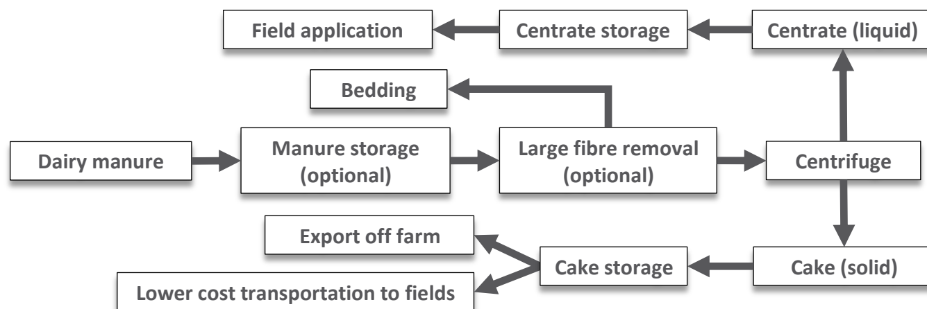
Figure 2: Centrifuge Flow Diagram for a Dairy Farm
