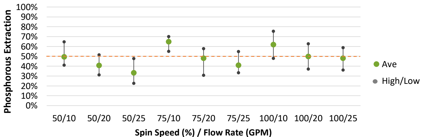
Graph 2: P Extraction from Processed Manure (scrape barns)
